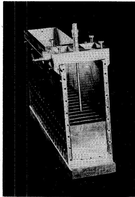
Fig. 1. An overdimensioned rectangular periodic waveguide.
