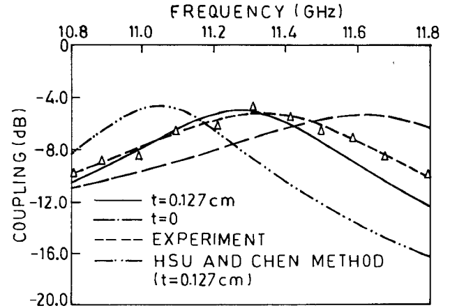
Fig. 4. Variation of coupling with frequency for 2L = 1.4 cm and 2W = 0.08 cm.
