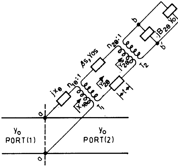
Fig. 2. Equivalent network representation.
