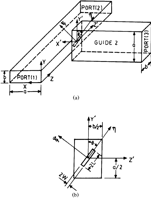
Fig. 1. Inclined slot-coupled coplanar E - H plane tee junction.
